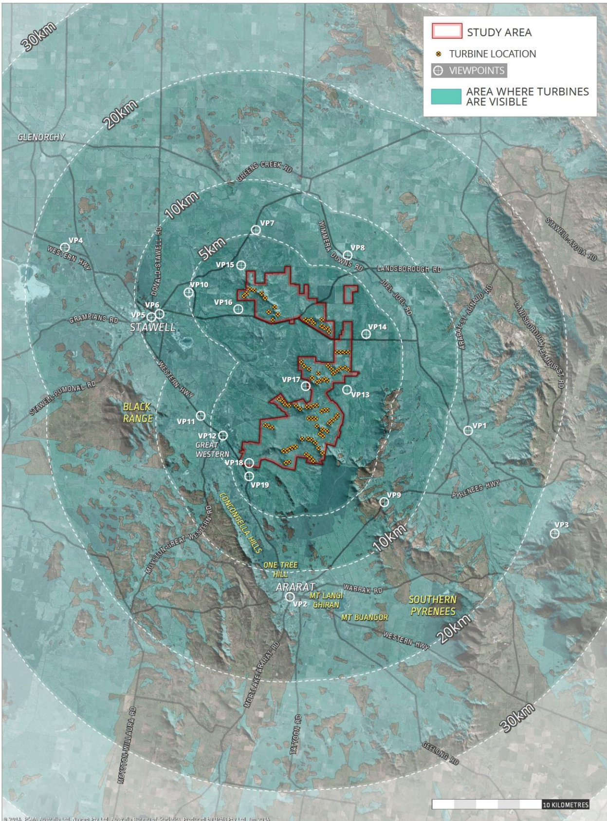
FIGURE 15 – PRELIMINARY TZVI ANALYSIS (BLADE TIP HEIGHT 196 METRES) AND KEY SENSITIVE VIEWPOINTS
